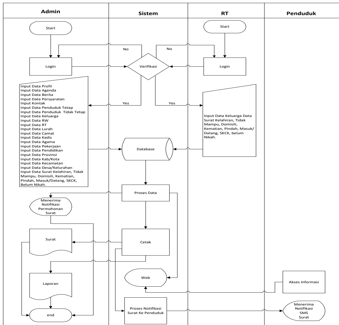
Gambar 3.1 flowchart sistem
