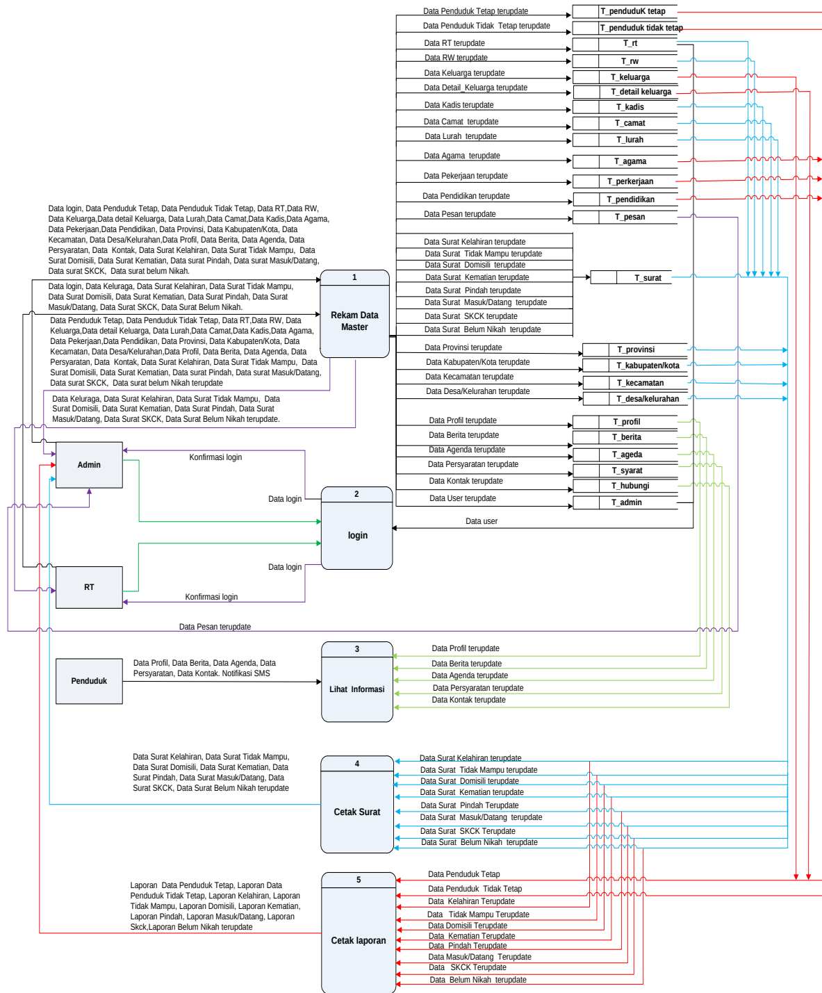
Gambar 3.3 Diagram Level 1
